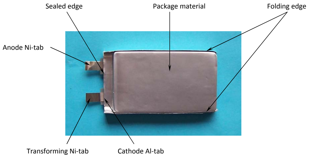
Fig.1. Exterior schematic of polymer lithium-ion cells
