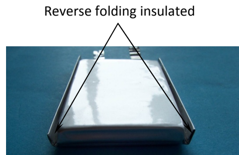
Fig.3. Reverse folding edge schematic of PL cells
