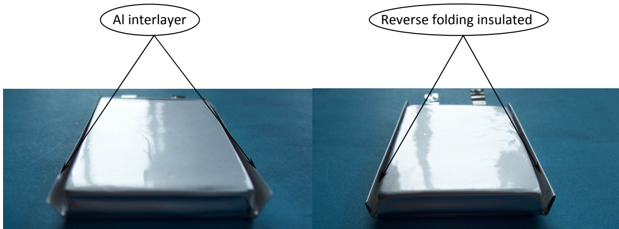
Fig.2. Single folding edge schematic of PL cells
